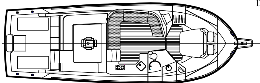
Single Stateroom Plan
