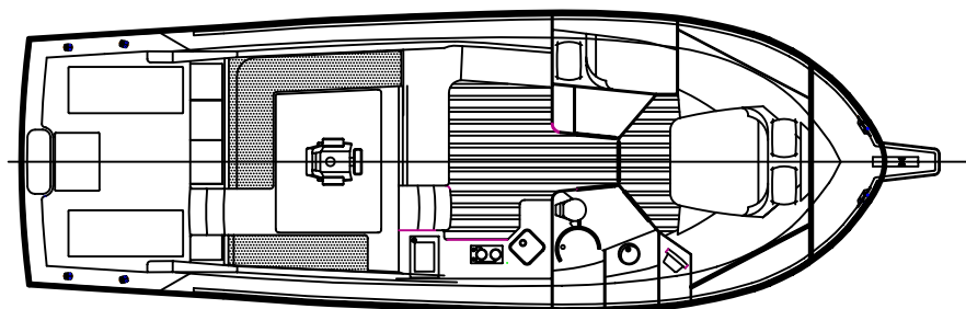
Double Stateroom Plan
